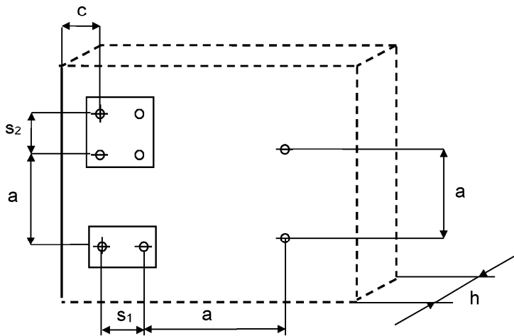
Scheme of distance and spacing in autoclaved aerated concrete – base material group “d”
